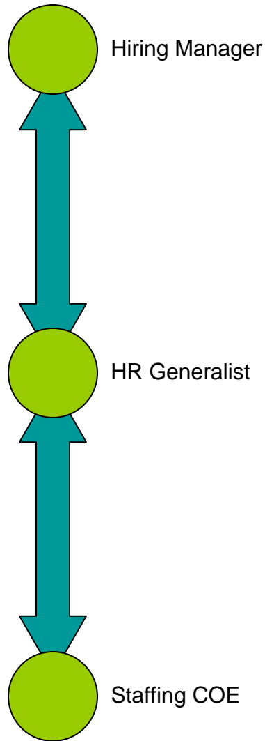
Figure 1: Broker Method
